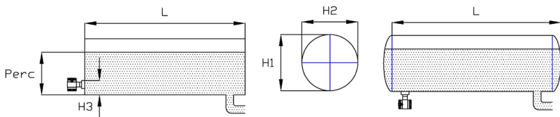
Cylindrical horizontal tank
