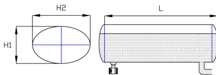
Cylindrical tank with cone-shaped ends
